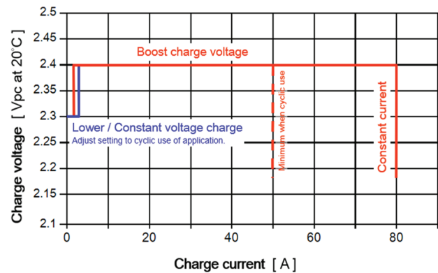
Figure 3: Charging characteristic IU0U charge for ZeMa200P18*
