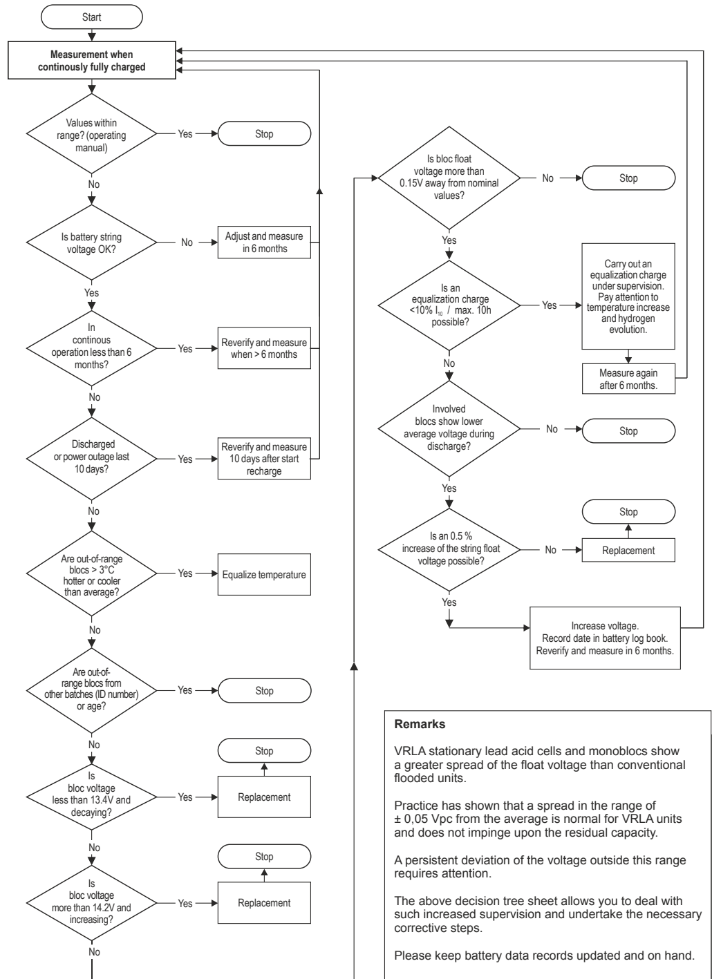
Decision tree for the analysis of voltage deviations (12V monoblocs under continuous charge)
